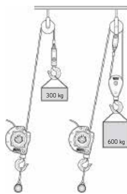
PULLEYMAN fixed to the floor
