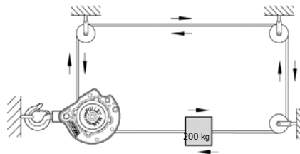
Fixed PULLEYMAN moving rope, load direction straight and inclined
