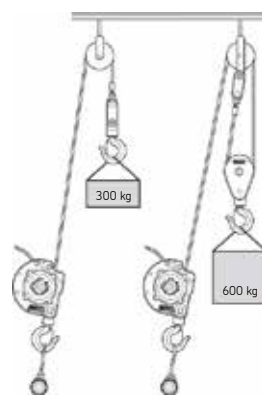
PULLEYMAN fixed to the floor
